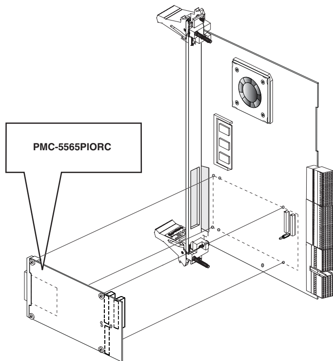
Figure 1-3 Installing the PMC-5565PIORC
