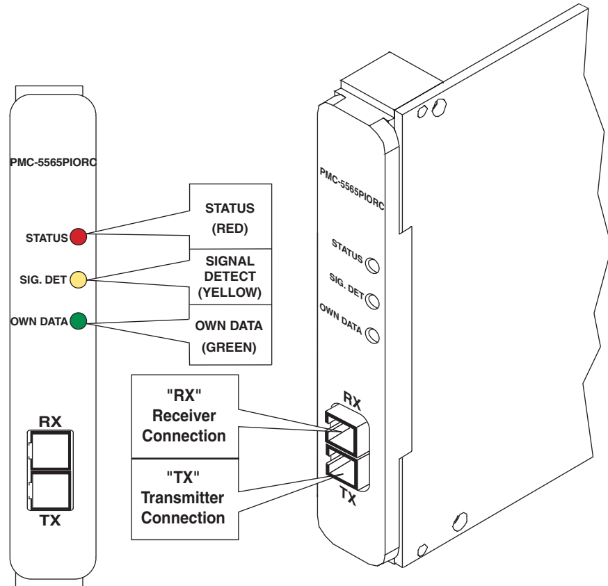
Figure 1-4 Front Panel of PMC-5565PIORC
