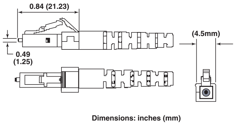
Figure 1-5 LC Type Fiber-Optic Cable Connector)
