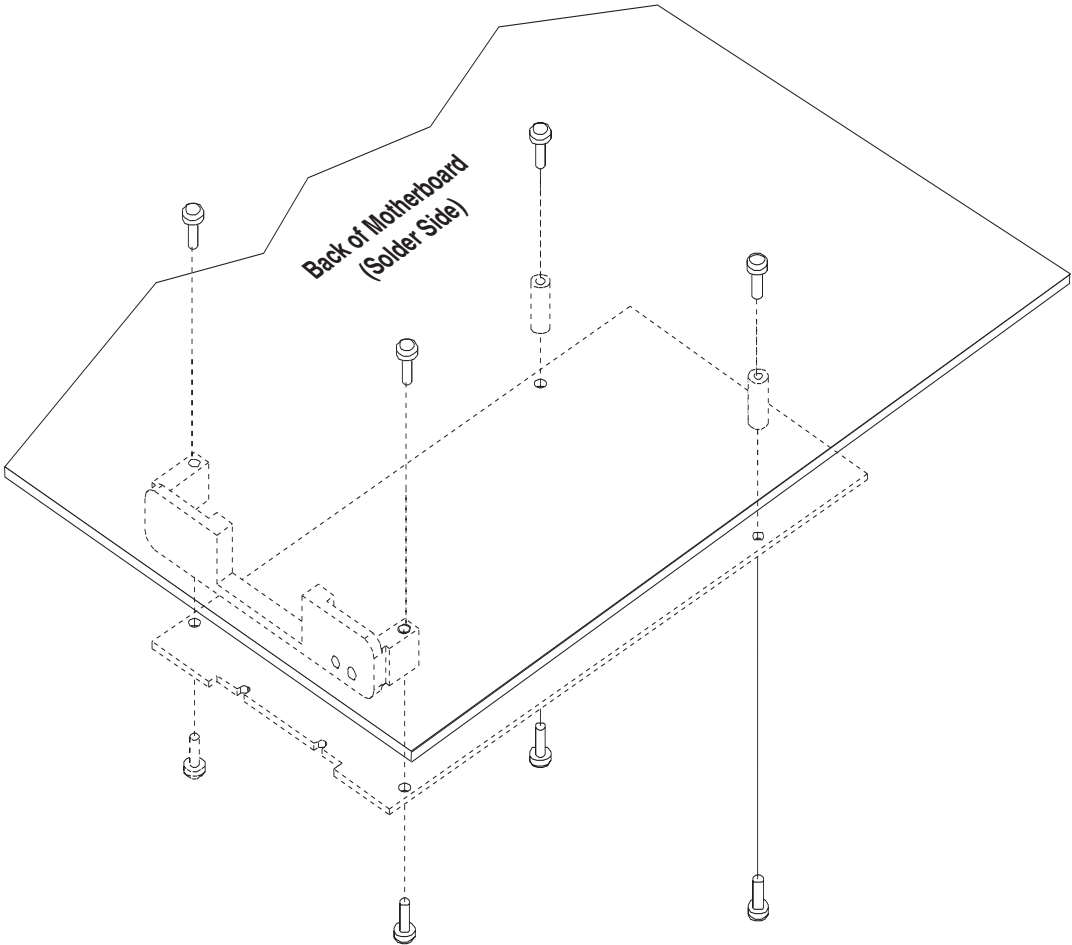
Figure 1-2 Backside Mounting of the PMC-5565PIORC
