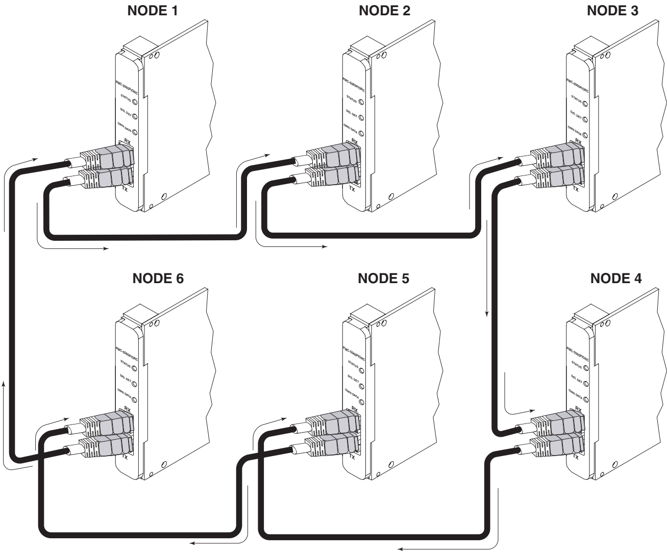
Figure 1-6 Example: Six Node Ring Connectivity PMC-5565PIORC
