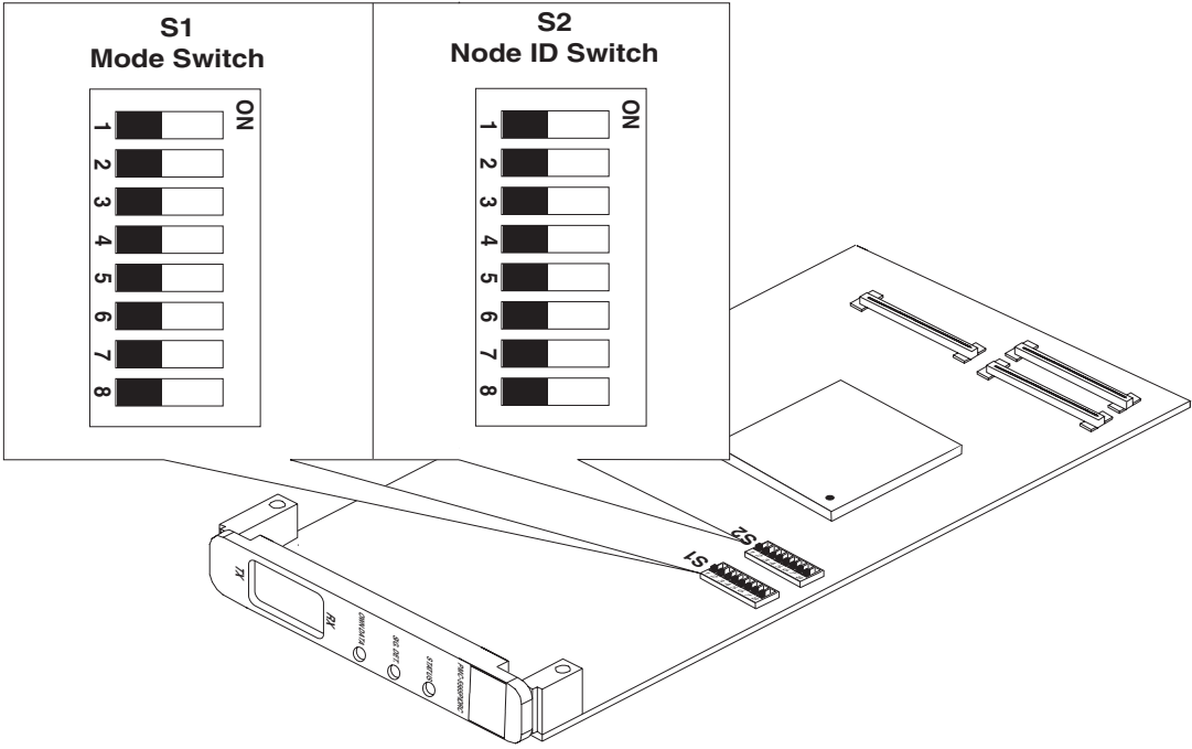
Figure 1-2 Backside Mounting of the PMC-5565PIORC
