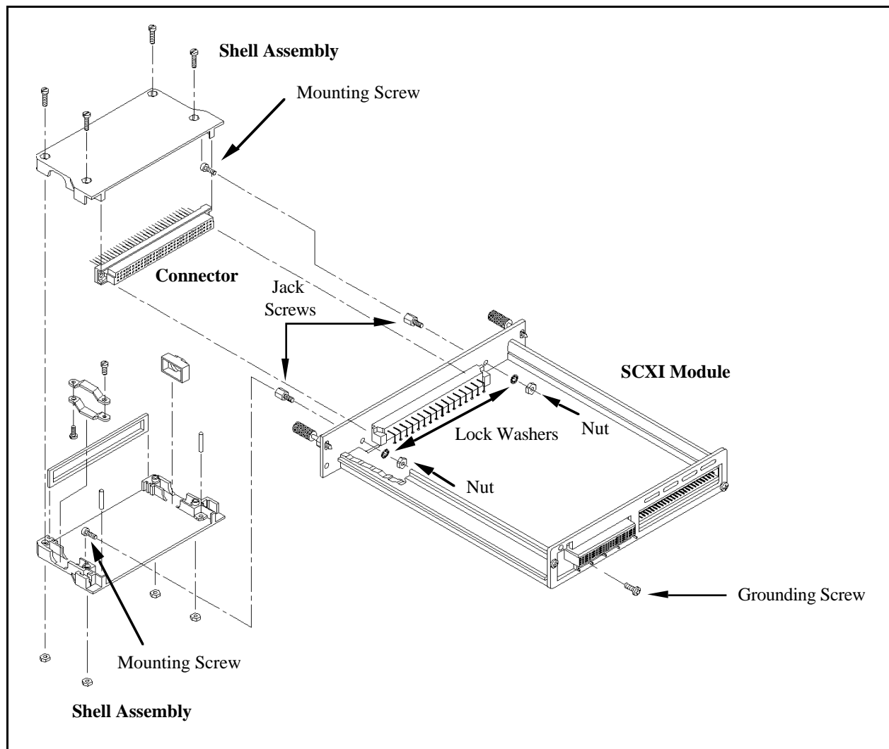
Figure 3-11. Building and Mounting the SCXI-1310 or SCXI-1330 Connector-and-Shell Assembly
