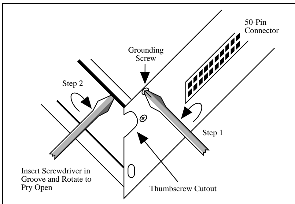
Figure 2-7. Cover Removal
