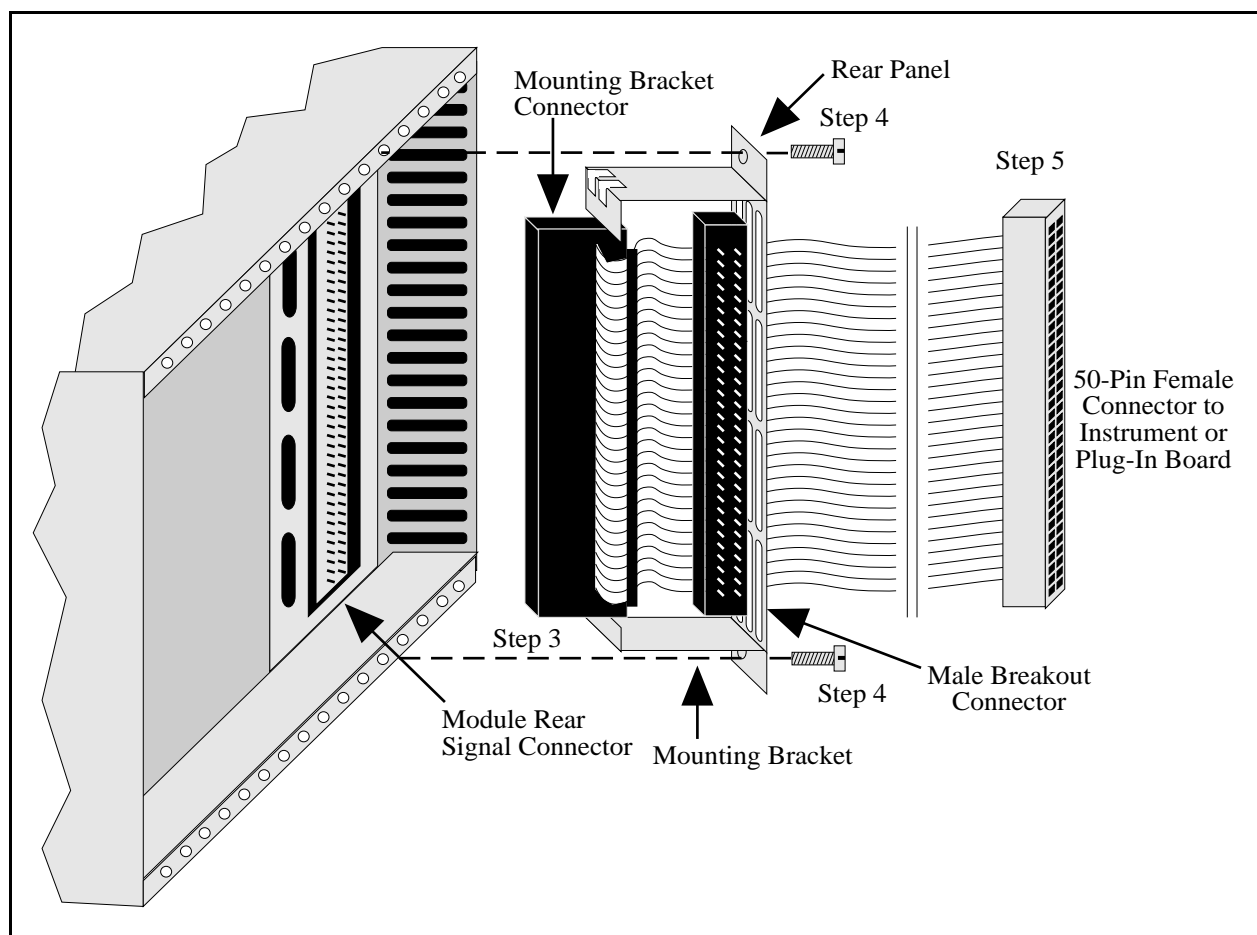
Figure A-1. SCXI-1340 Installation
