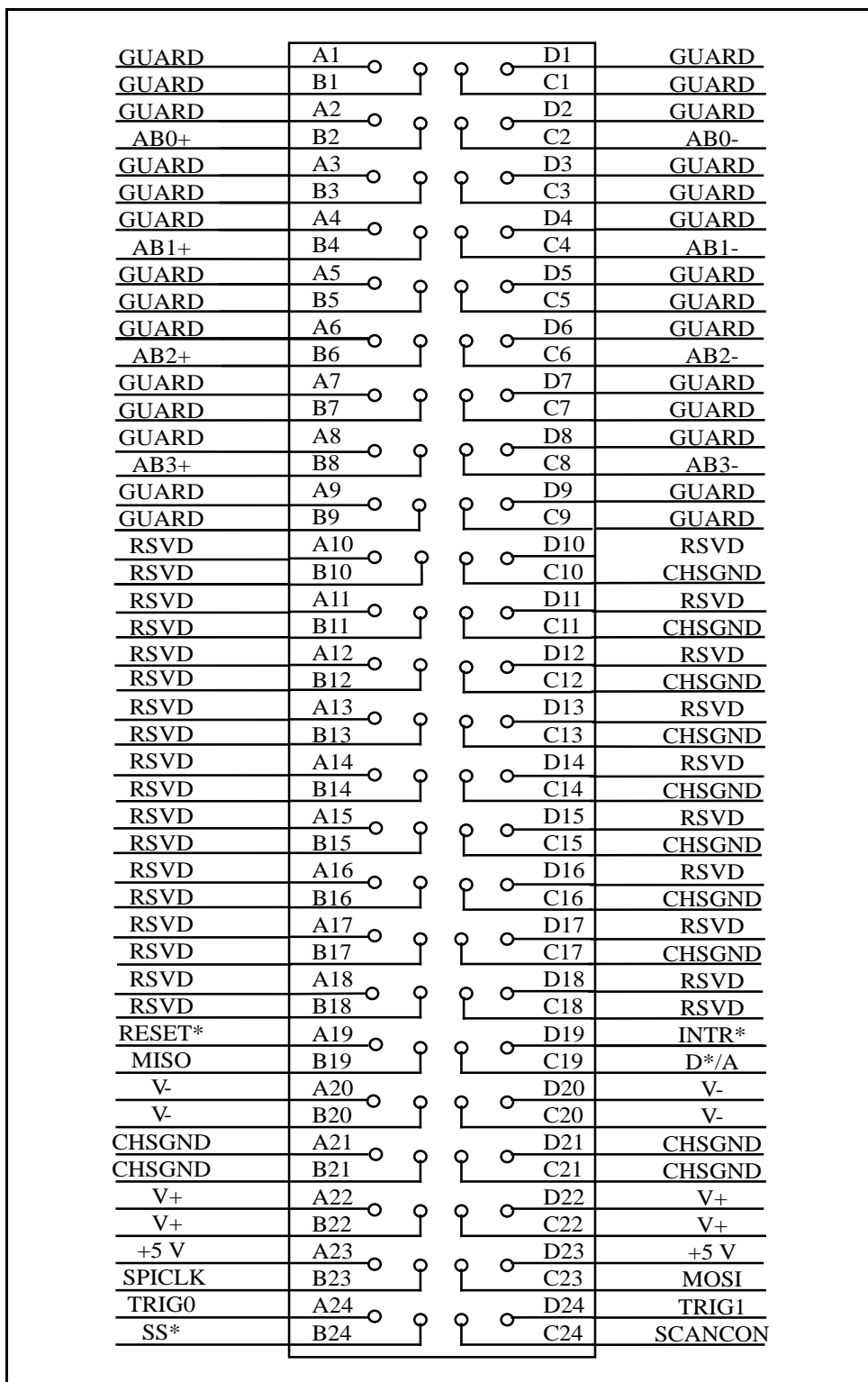
Figure 3-3. SCXI-1181 SCXIBus Connector Pin Assignment
