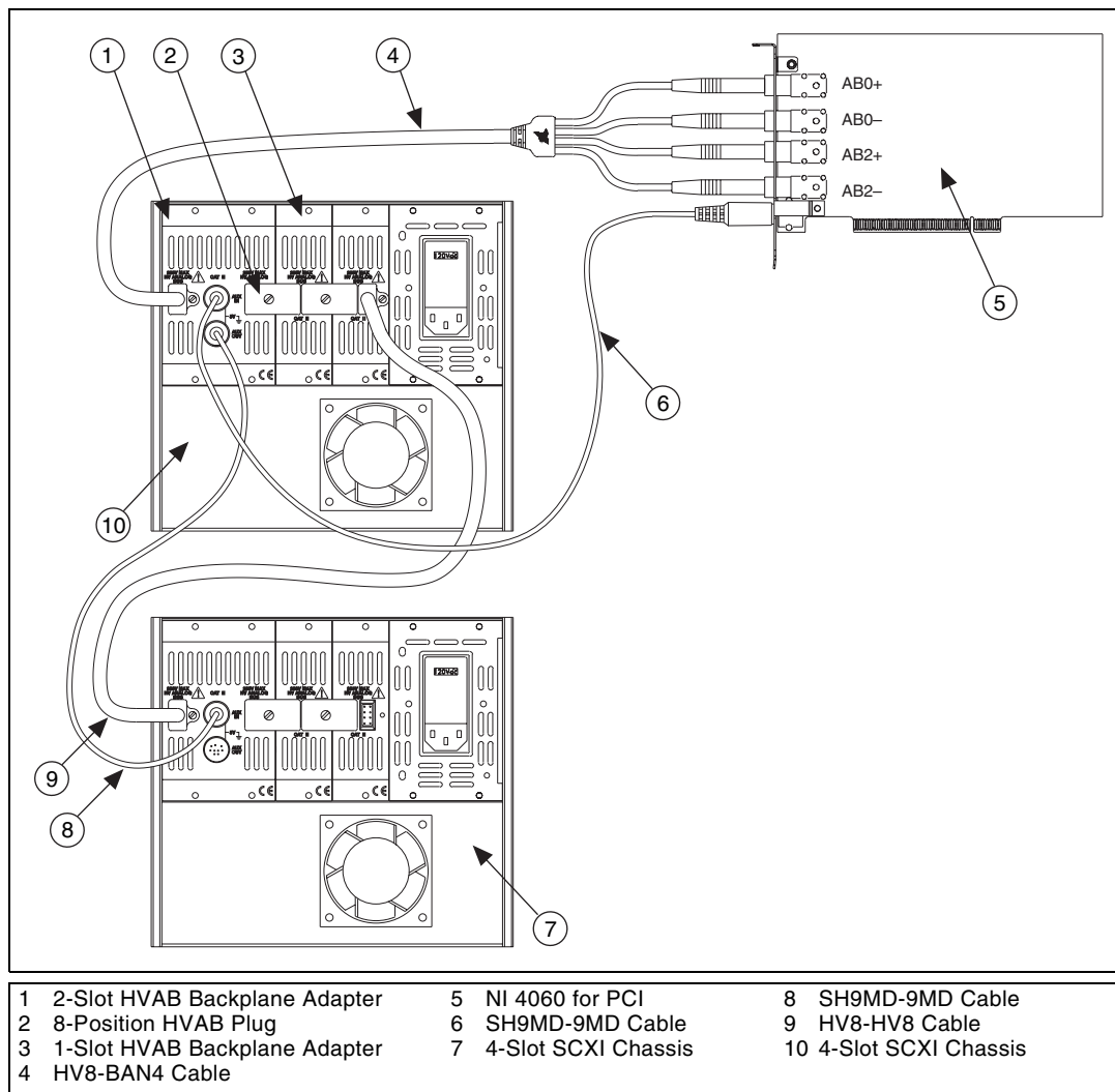
Figure 1-4. 4-Slot to 4-Slot Multichassis Configuration Parts Locator Diagram
