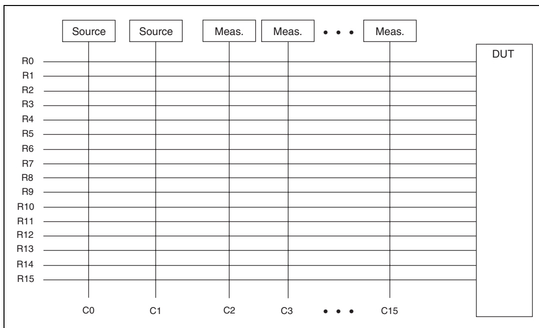
Figure 2-9. 16 × 16 Matrix Test Setup Example
