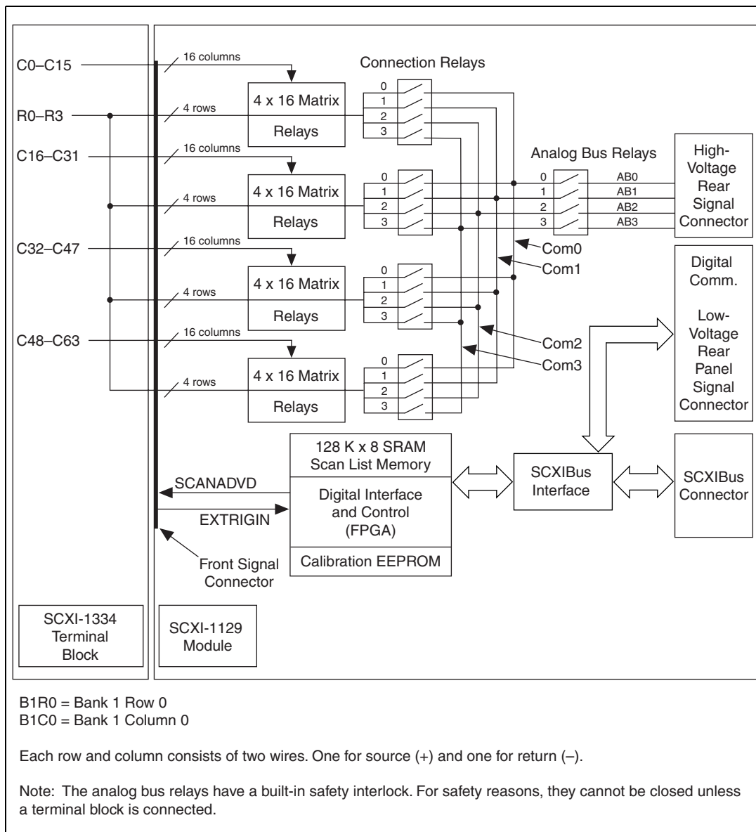
Figure 2-7. 4 × 64 Matrix Configuration
