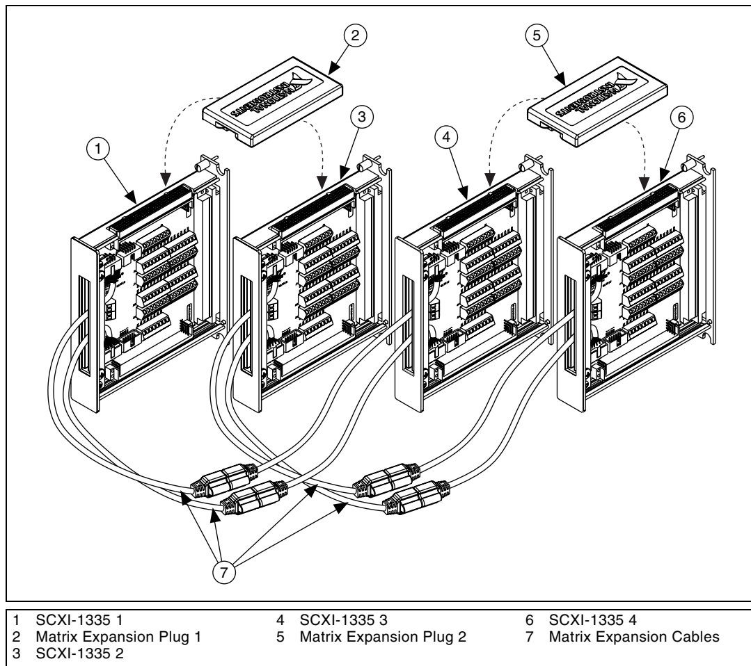
Figure 2-13. Example of Column and Row Expansion Using SCXI-1335 Modules
