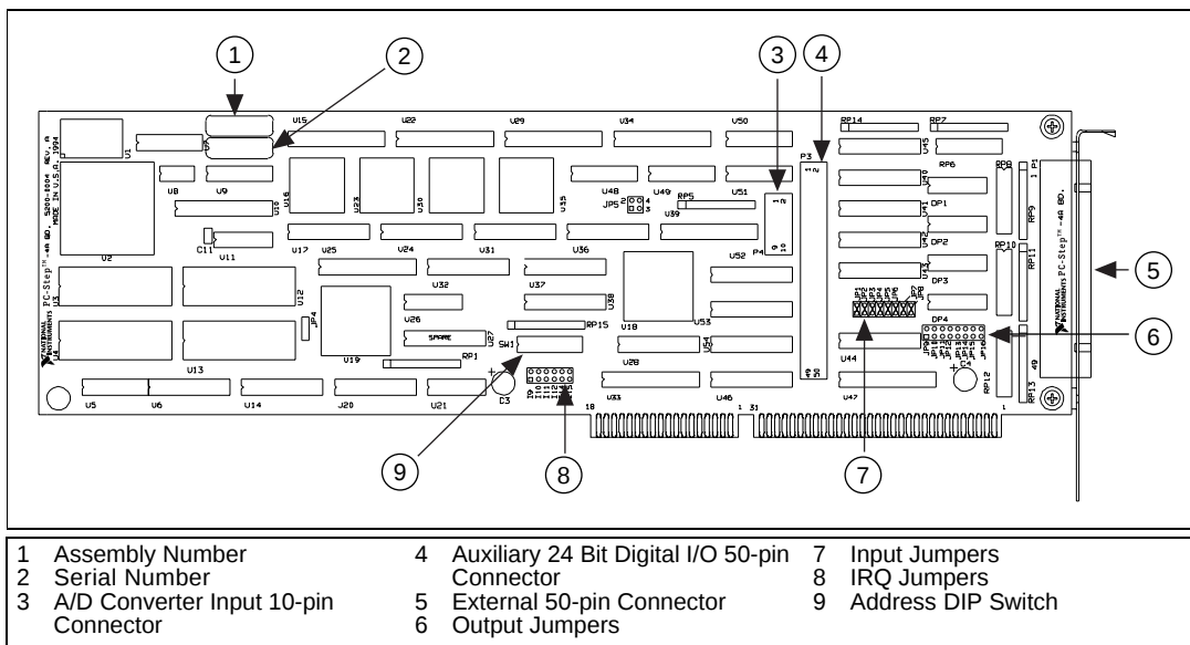
Figure 3-2. PC-Step Parts Locator Diagram
