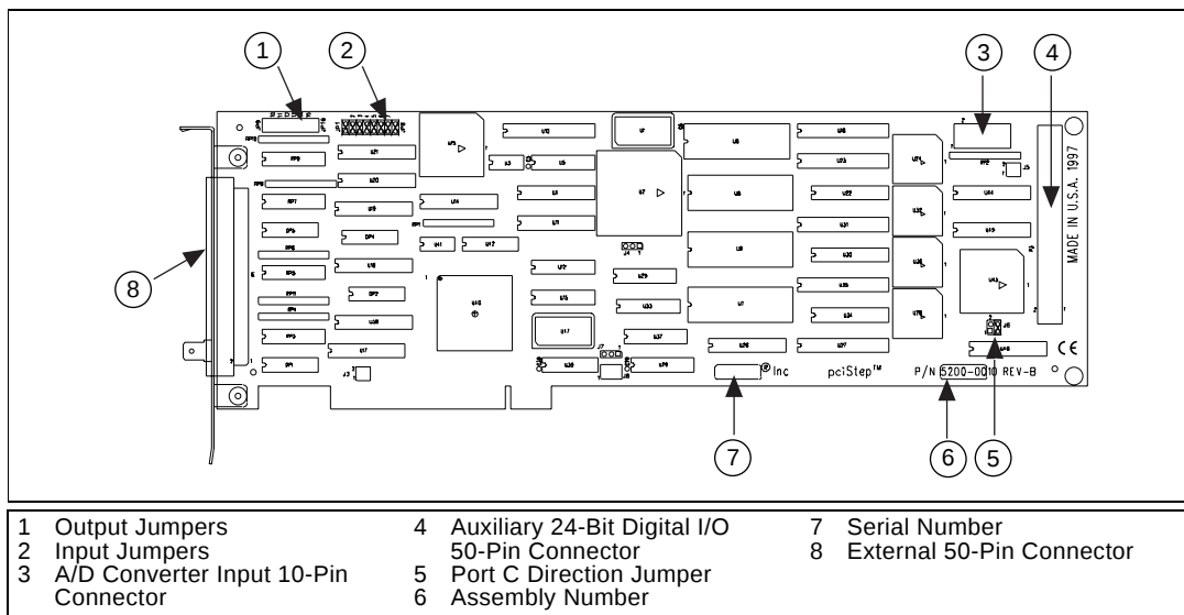
Figure 3-4. PCI-Step Parts Locator Diagram
